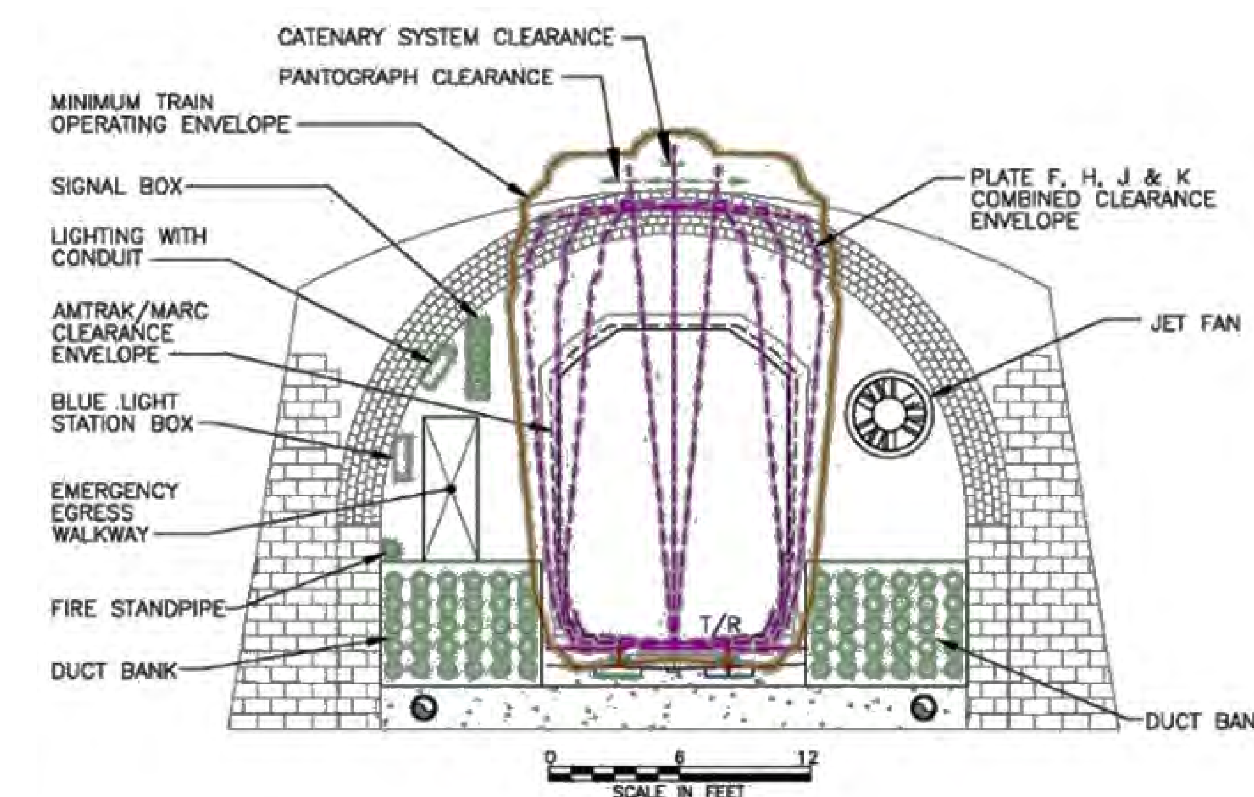
Single-Track Concept
