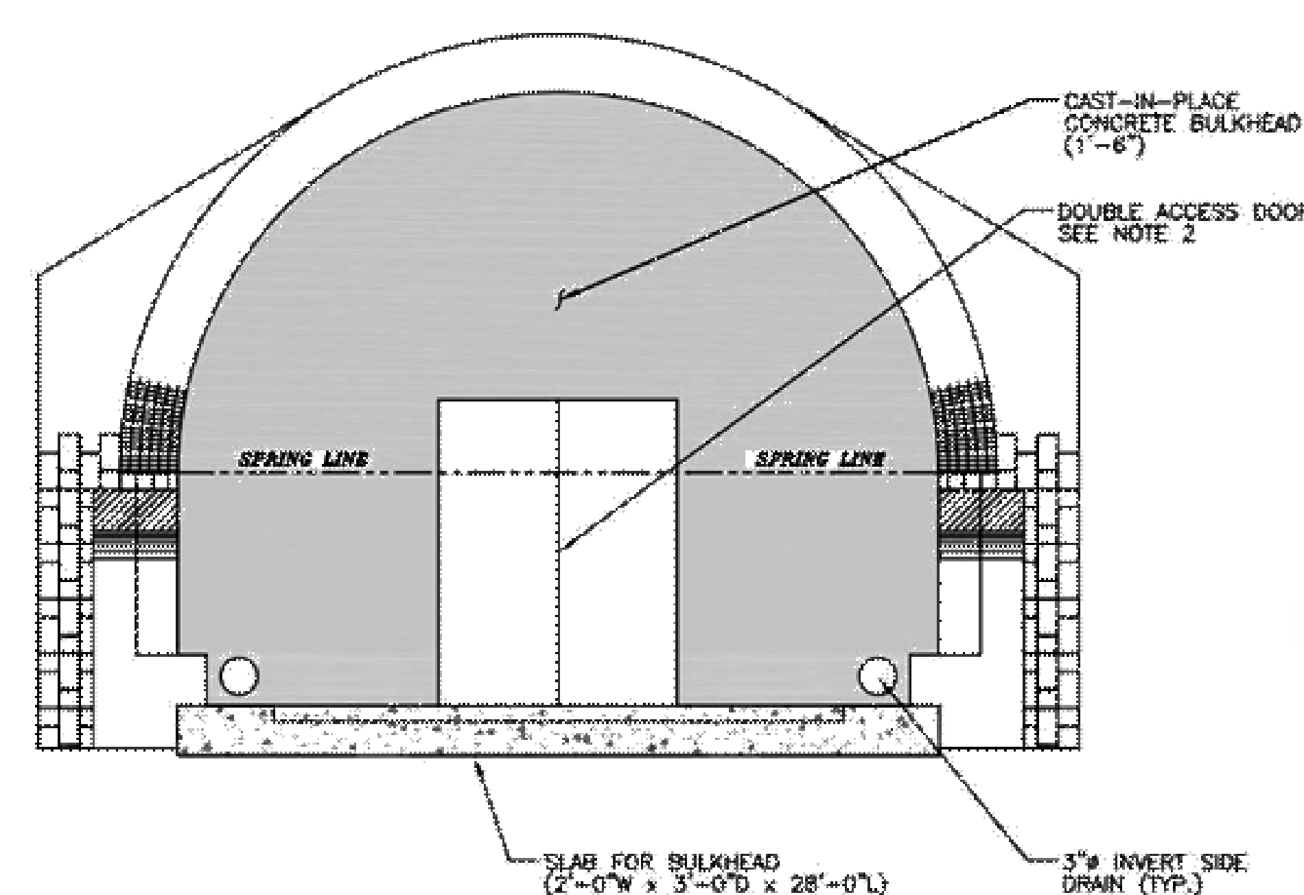
Abandonment Concept
