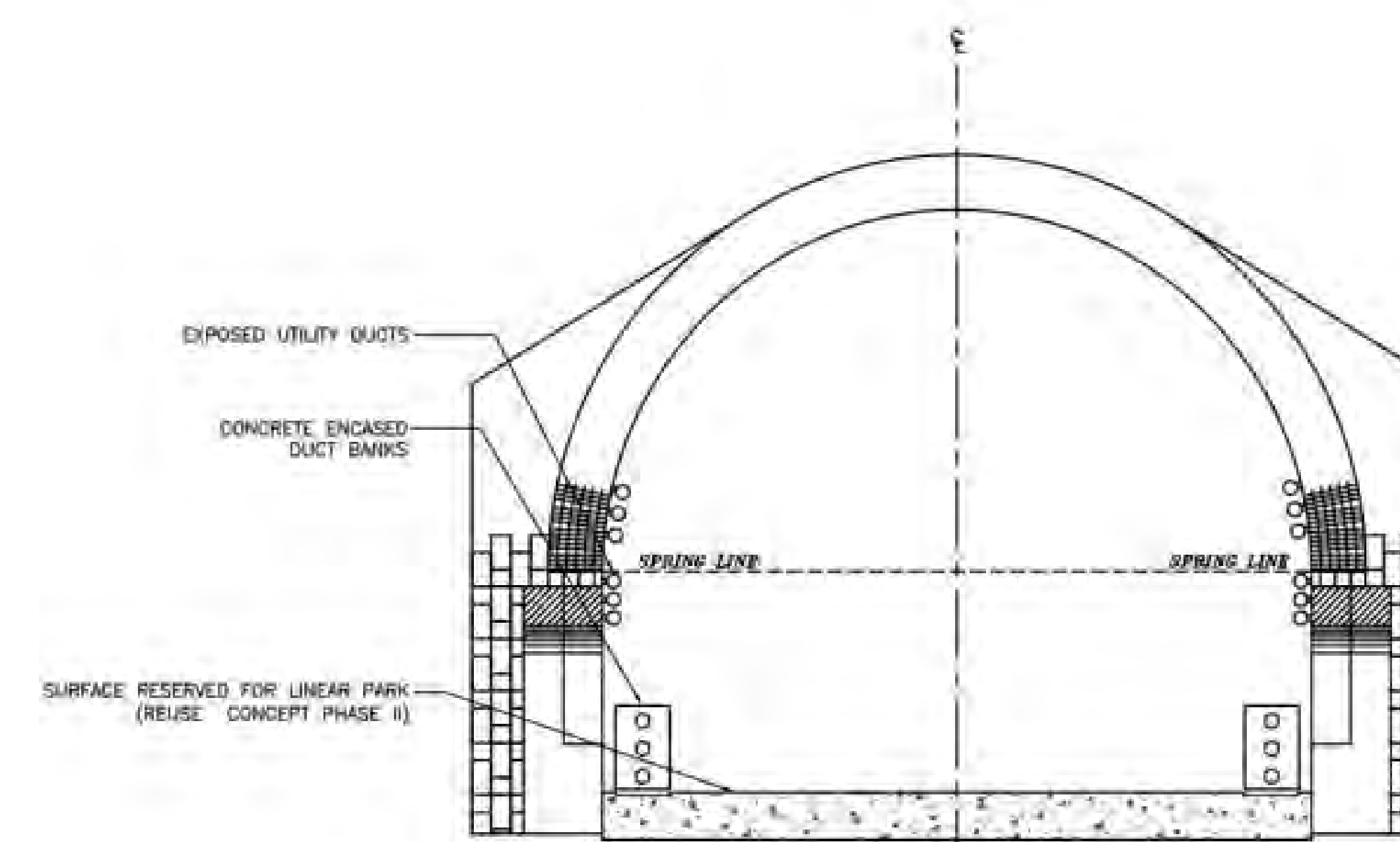
Utility Corridor
